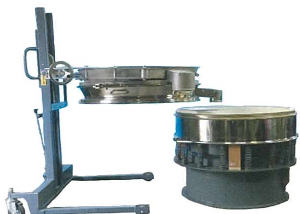
③ MOVE
